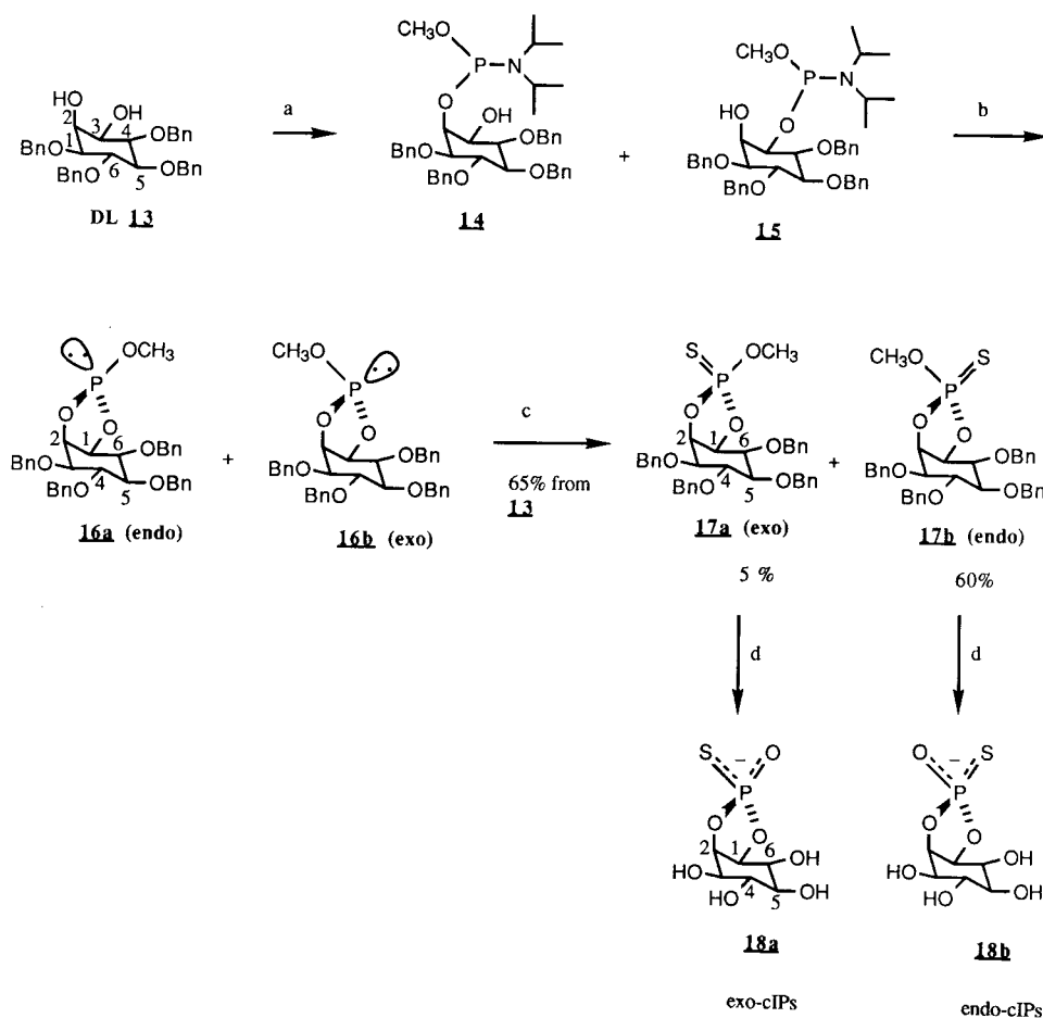
Scheme II: Synthesis of exo - and endo -cIPs a
