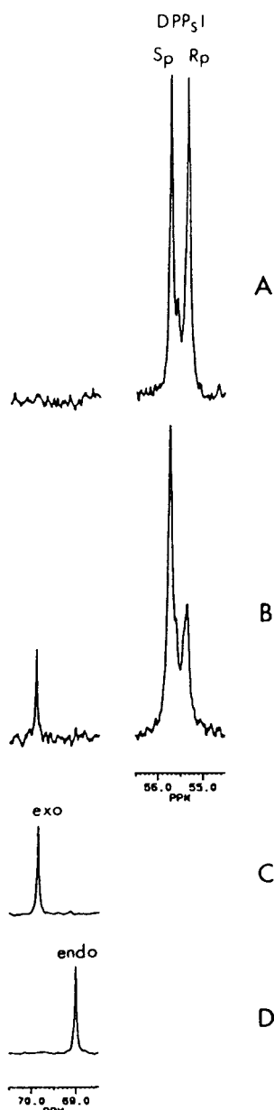
FIGURE 2: Use of ^{31}\text{P} NMR (101.2 MHz) to show the stereospecificity of PI-PLC. (A) 7.5 mg of ( R_p+S_p )-DPPsI in 50% \text{D}_2\text{O} containing 5% Triton X-100, 50 mM HEPES buffer, pH 7.2, 2.5 mM \text{Ca}^{2+} , and 0.25 mM EDTA. (B) 72 h after addition of 2 mg of PI-PLC from B. cereus . (C) 18a ( exo -DL-cIPs). (D) 18b ( endo -DL-cIPs).
