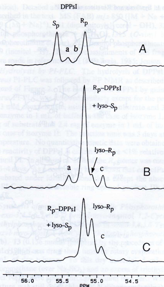
FIGURE 1: Use of 31 P NMR to monitor the hydrolysis of DPPsI by PLA 2 . (A) 10 mg of ( R p + S p )-DPPsI in 50% D 2 O containing 5% Triton X-100, 50 mM HEPES buffer, pH 7.2, 2.5 mM Ca 2+ , and 0.25 mM EDTA. (B) Spectrum taken within the first 30 min after addition of 1.3 mg of PLA 2 from bee venom. (C) After further incubation at 25 °C for 12 h.
