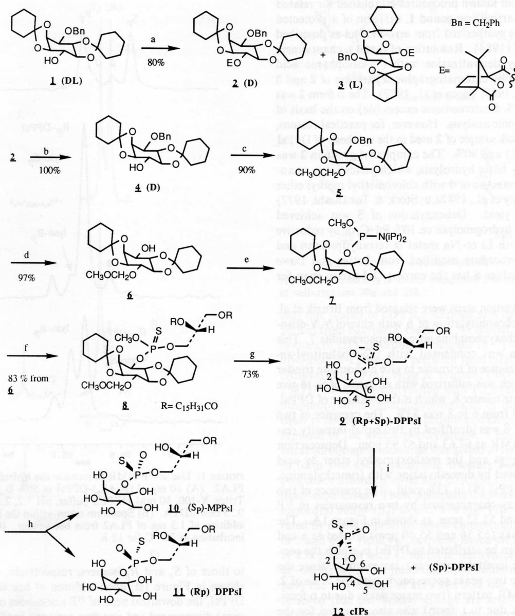
Scheme I: Synthesis and Reactions of DPPsI a
