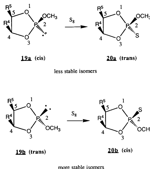
FIGURE 3: Structures of model phosphites 19a and 19b and products of sulfurization 20a and 20b .
